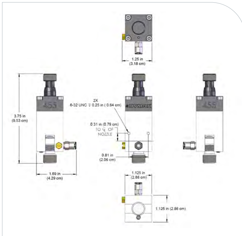
Figure 1. Model 455 Dimensions
