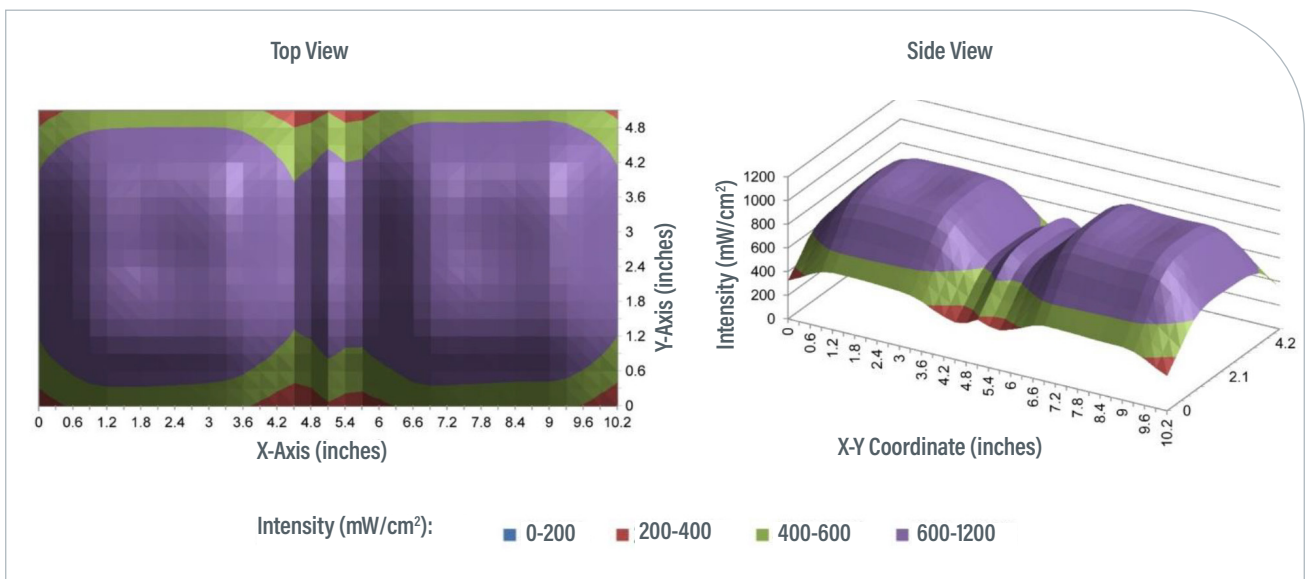
Figure 1. Intensity Distribution of Two BlueWave LED Flood VisiCure Arrays (405 nm) Mounted Side-by-Side
