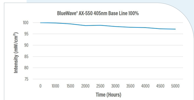
Figure 7. LED Degradation Testing - VisiCure®
