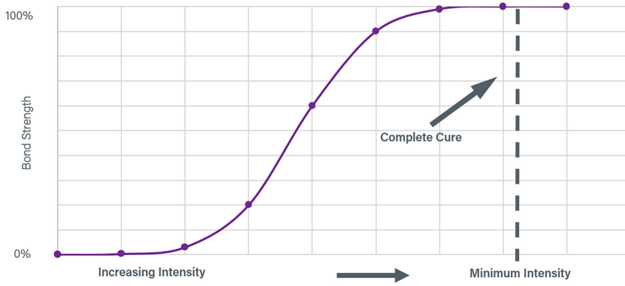
Figure 1. Curing Energy Profile (Exposure Time Held Constant)
