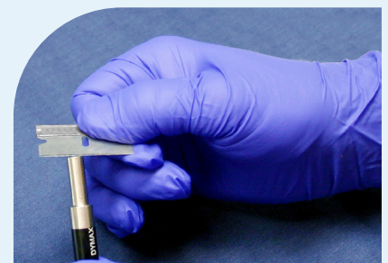
Figure 6. Clean Lightguide End With a Razorblade
